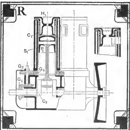
Fig. R—Longitudinal sectional view of the Carroll rotary sleeve valve motor and part section of a cylinder showing how the ports are uncovered
